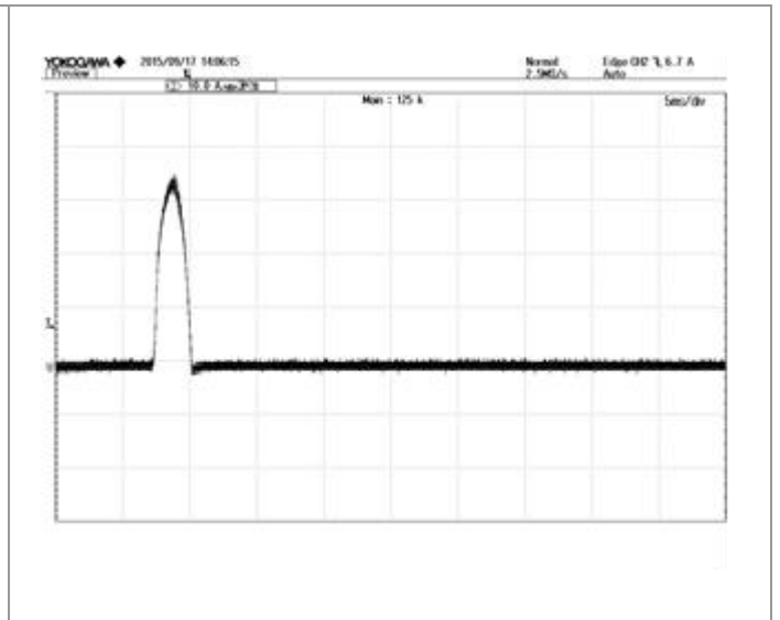
Figure 8: Inrush current @ Vin=220Vac. Iin: 10A/div, 5mS/div;
